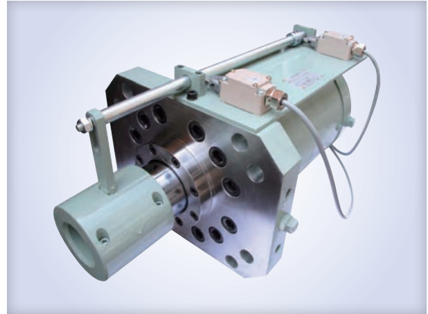
ELH Model FA Type (See P043) Accessories : Special MLS/Coupling/ Welded Type Arm
