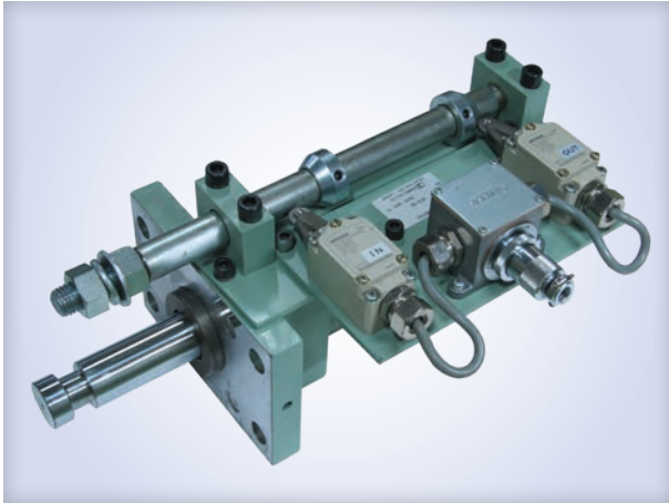
Standard Model FA Type (See P001) Accessories : HLS
